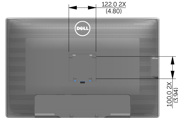
Back view of Monitor without stand
